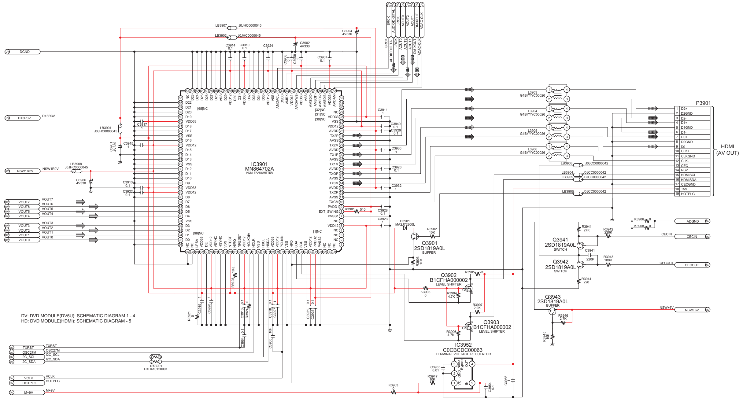
SA-PT875GA/GC/GS DVD MODULE(HDMI) CIRCUIT
