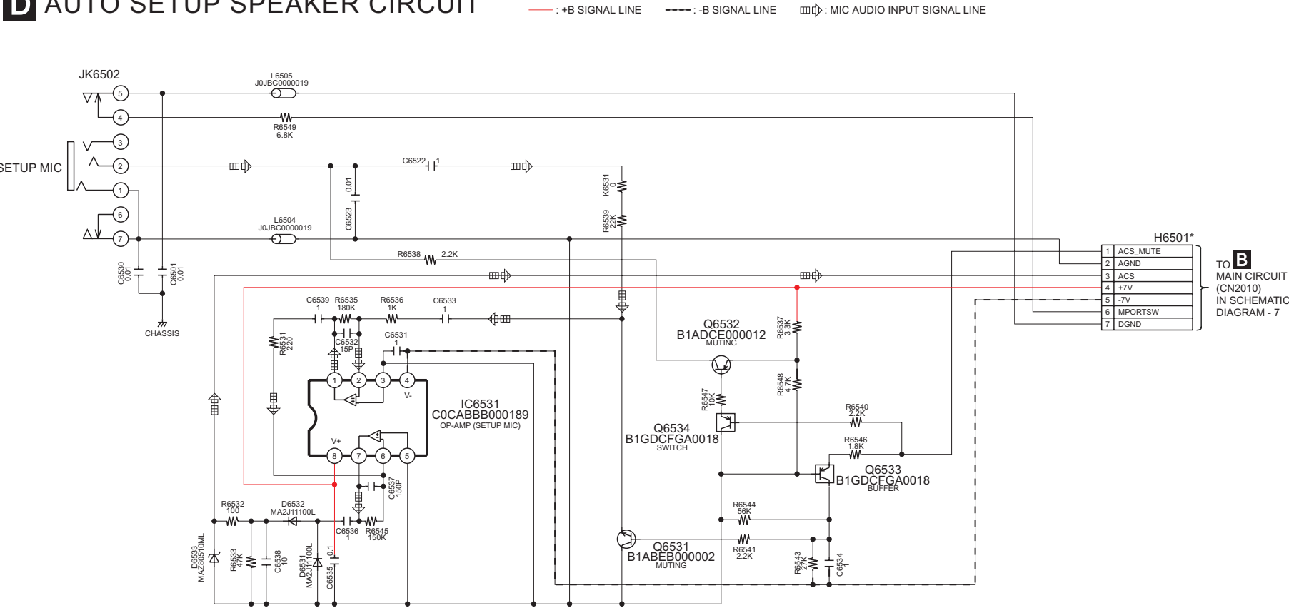
SCHEMATIC DIAGRAM - 11
