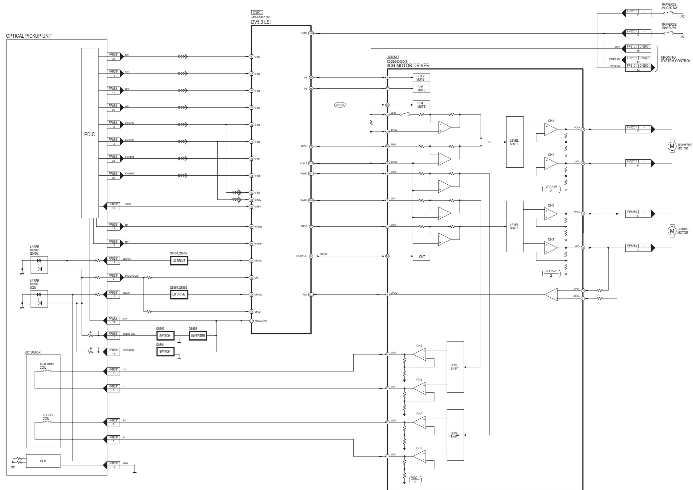
SA-PT875GA/GC/GS DVD (SERVO) BLOCK DIAGRAM
