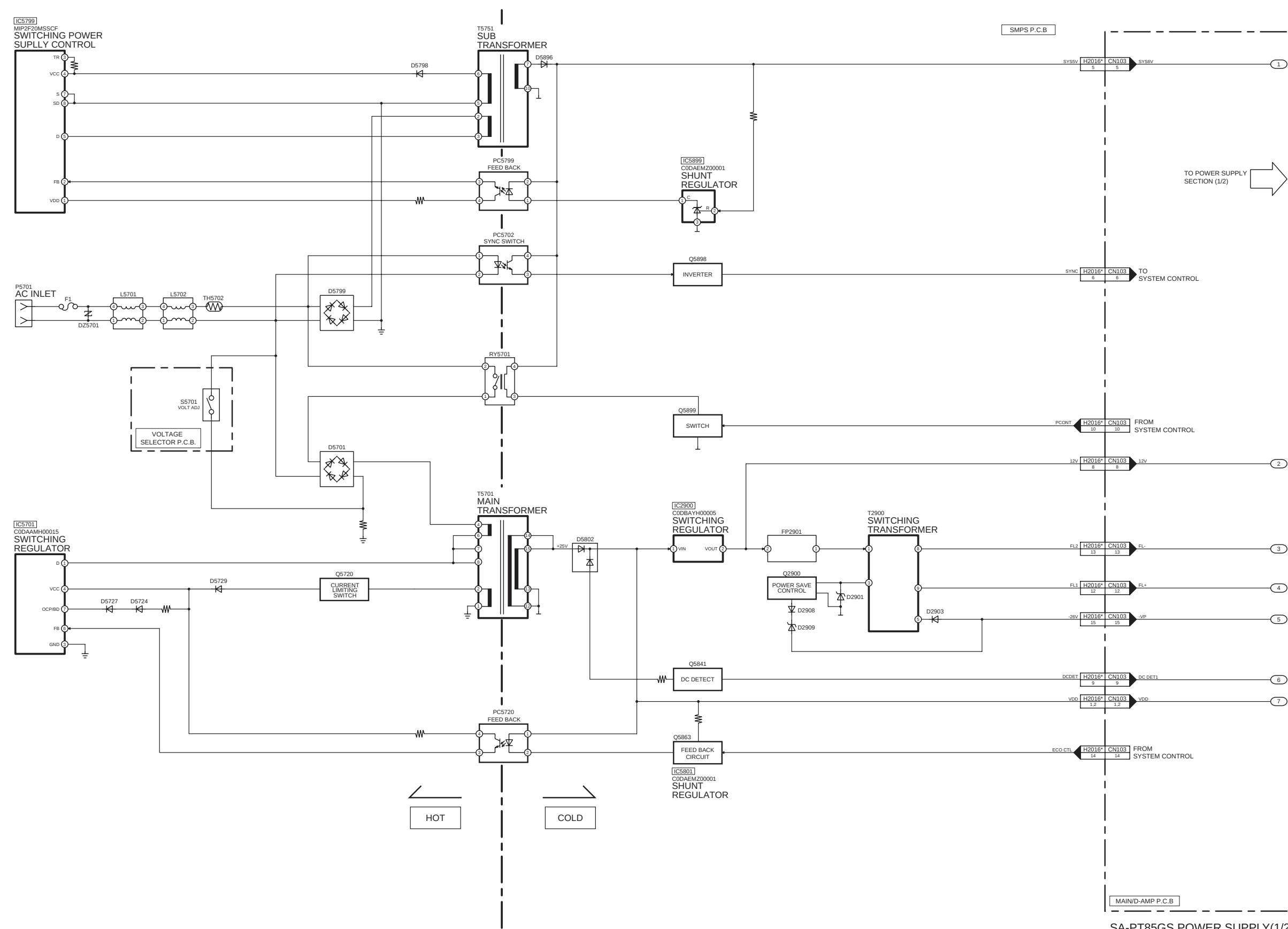
SA-PT85GS POWER SUPPLY(1/2) BLOCK DIAGRAM
