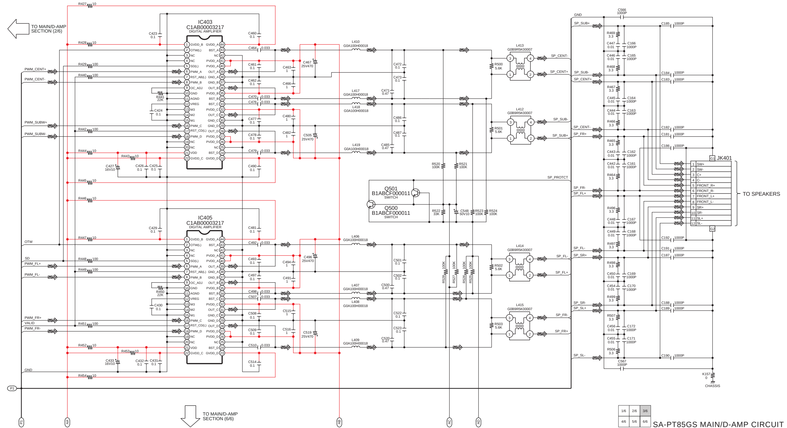
SA-PT85GS MAIN/D-AMP CIRCUIT
