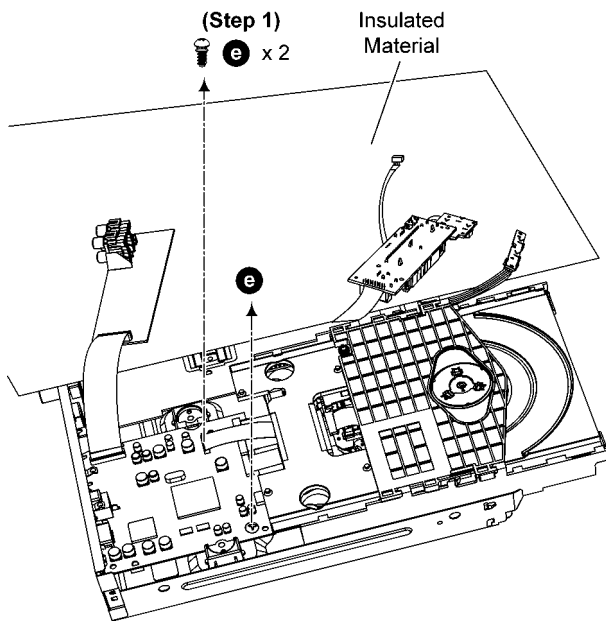
Step 1 Remove 2 screws.
