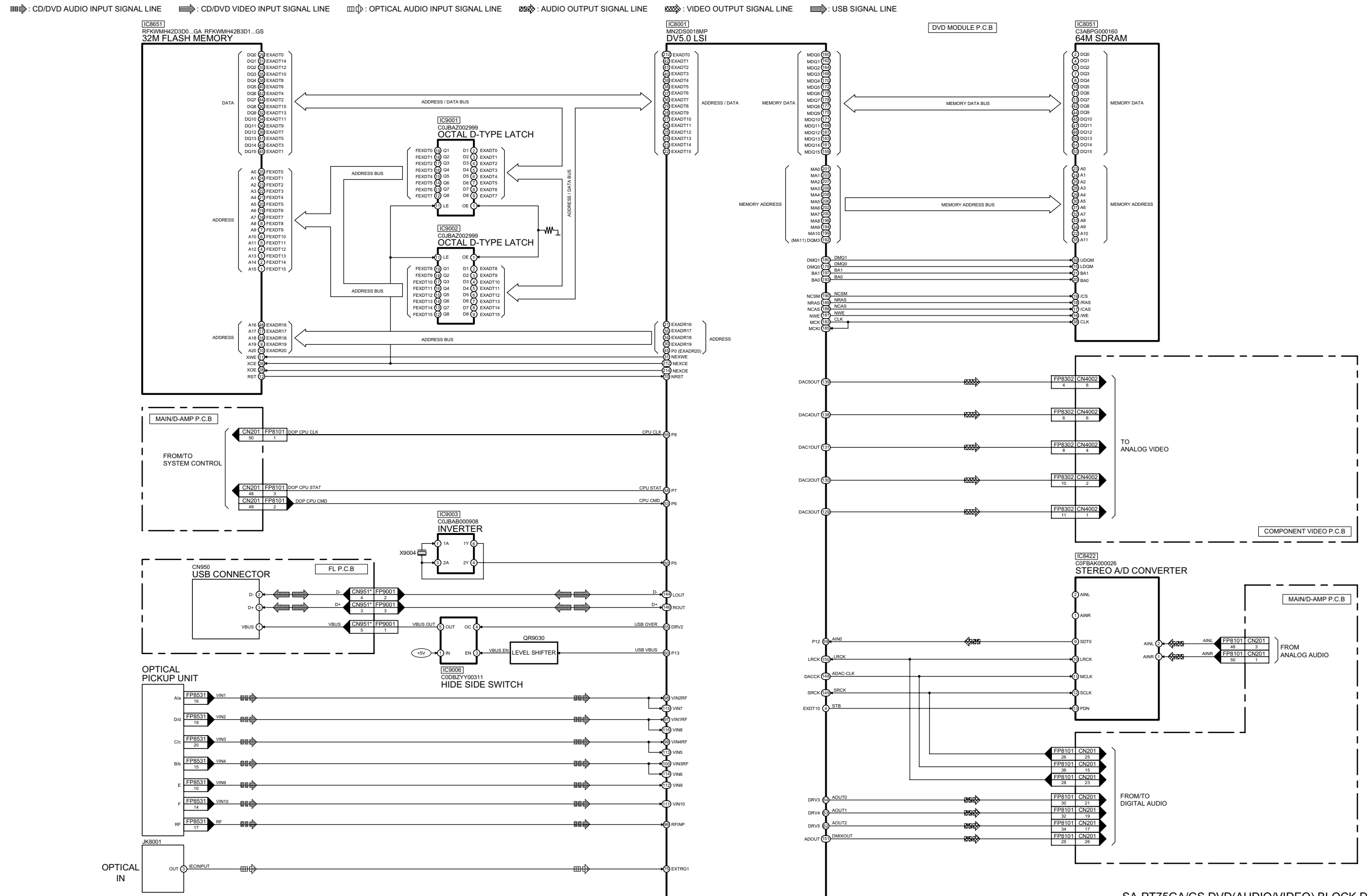
SA-PT75GA/GS DVD(AUDIO/VIDEO) BLOCK DIAGRAM
