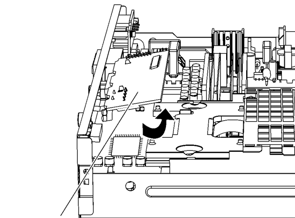
Component Video P.C.B. (Step 3)
