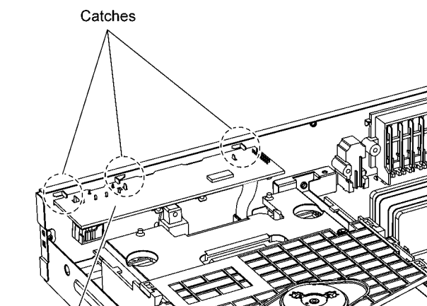
Component Video P.C.B.
