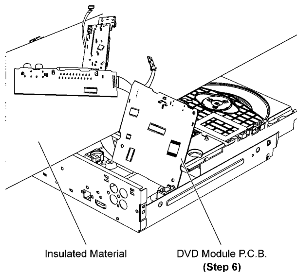
Step 6 Position DVD Module P.C.B. according to diagram shown.
