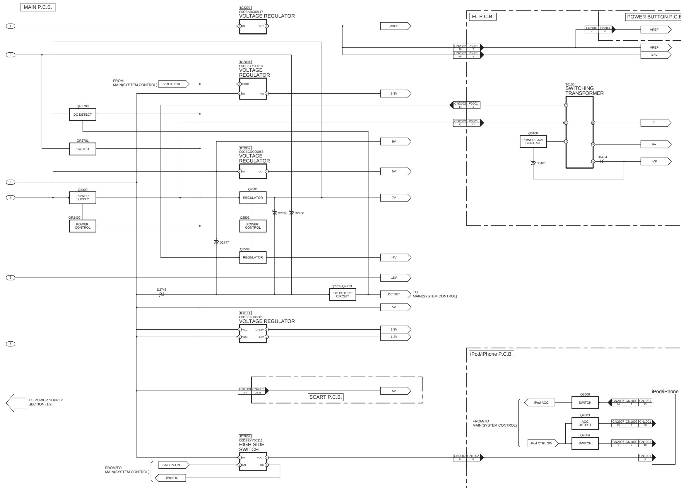
SA-PT580EB/EG/EP POWER SUPPLY(2/2) BLOCK DIAGRAM
