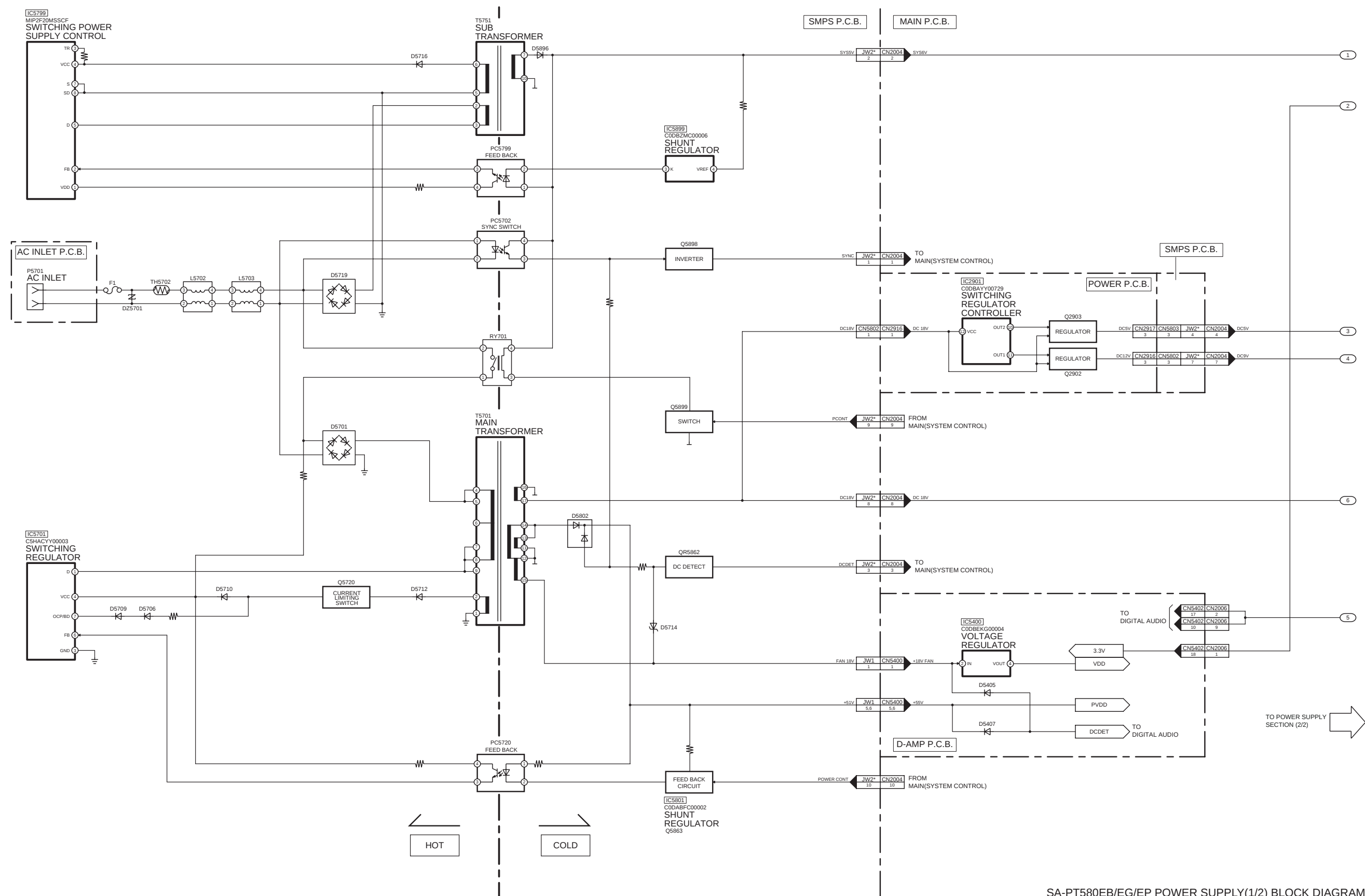
SA-PT580EB/EG/EP POWER SUPPLY(1/2) BLOCK DIAGRAM
