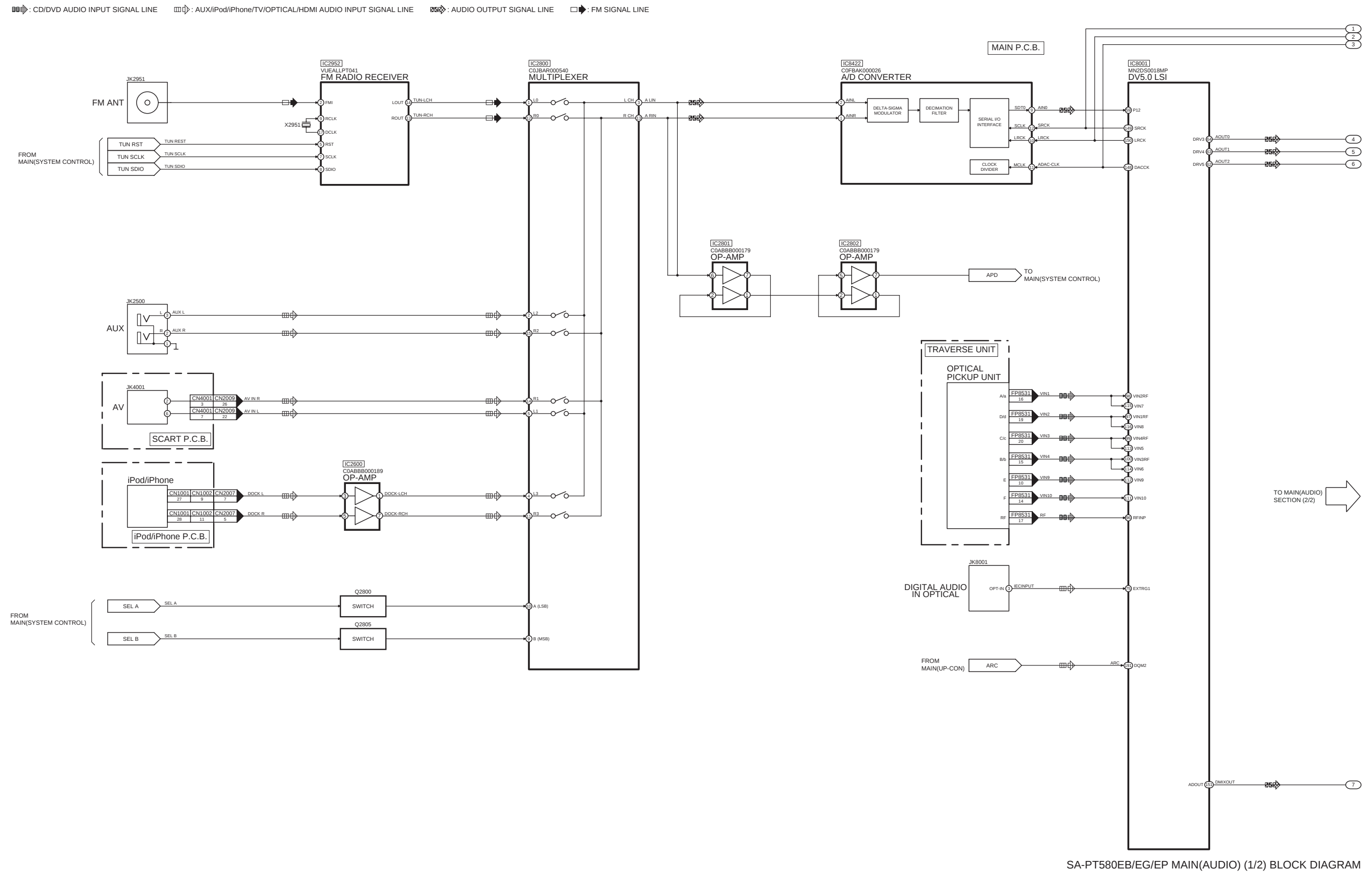
SA-PT580EB/EG/EP MAIN(AUDIO) (1/2) BLOCK DIAGRAM
