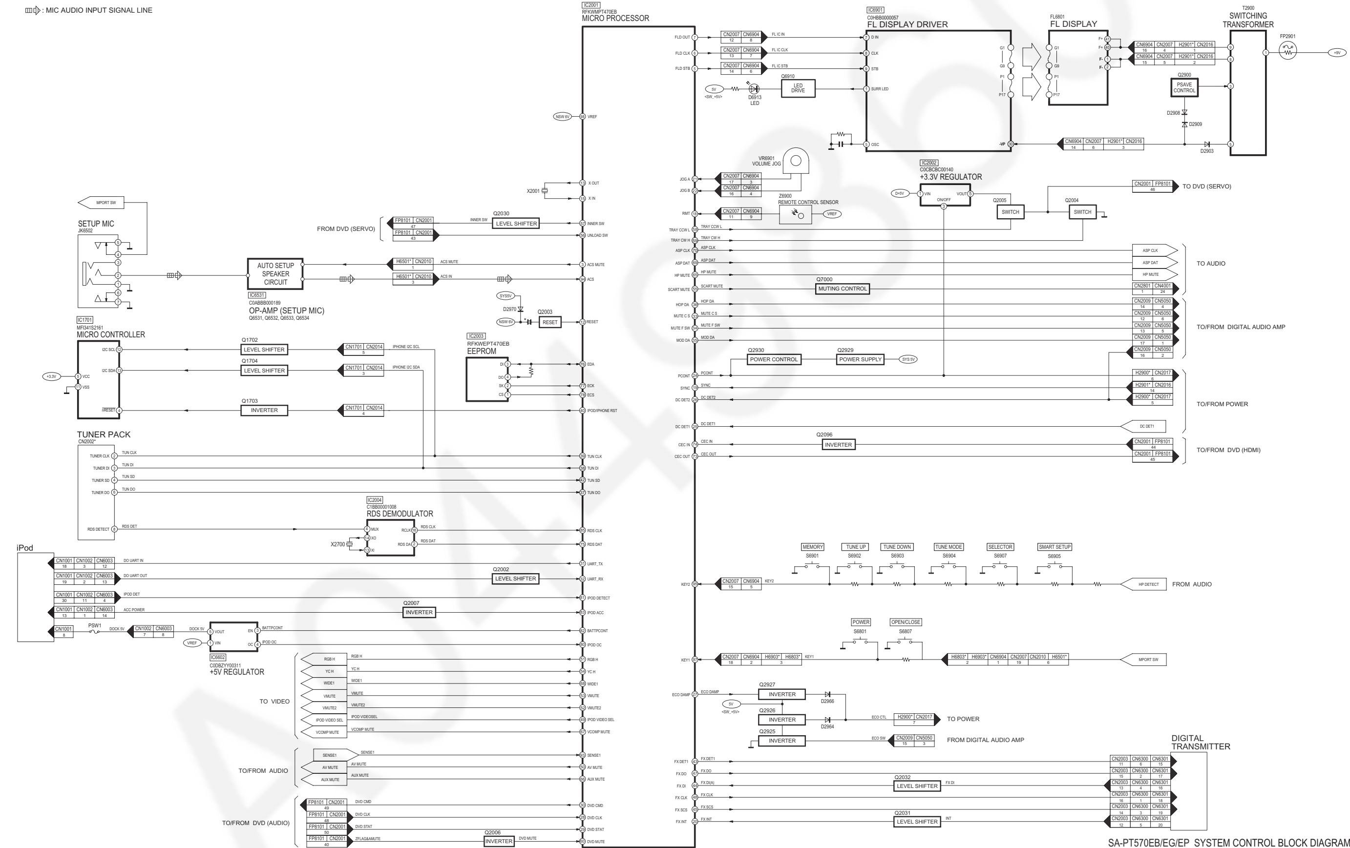
SA-PT570EB/EG/EP SYSTEM CONTROL BLOCK DIAGRAM
