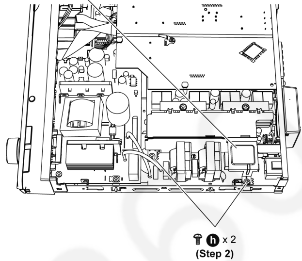
(Step 3) AC Inlet Shield Plate Unit
