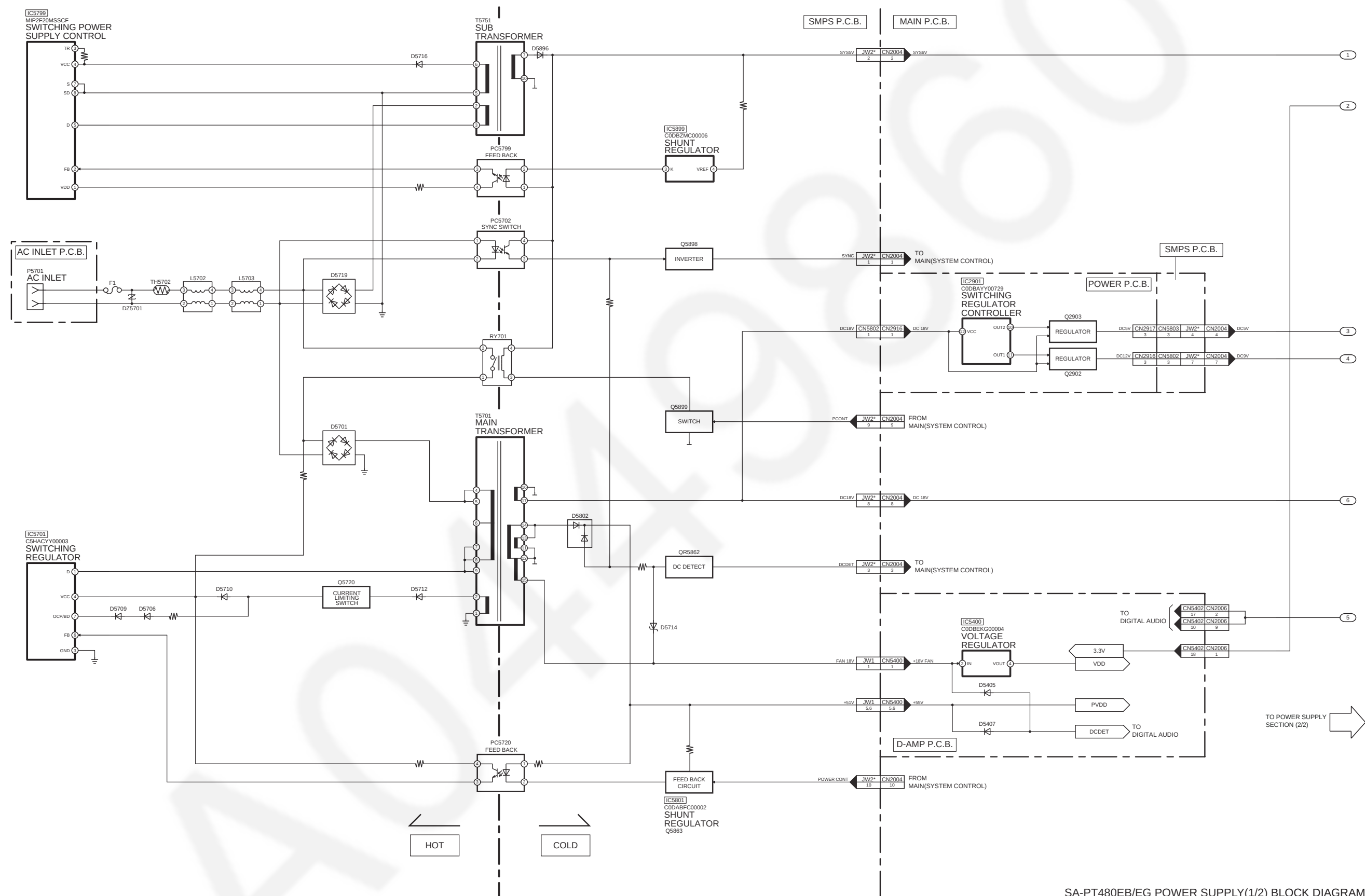
SA-PT480EB/EG POWER SUPPLY(1/2) BLOCK DIAGRAM
