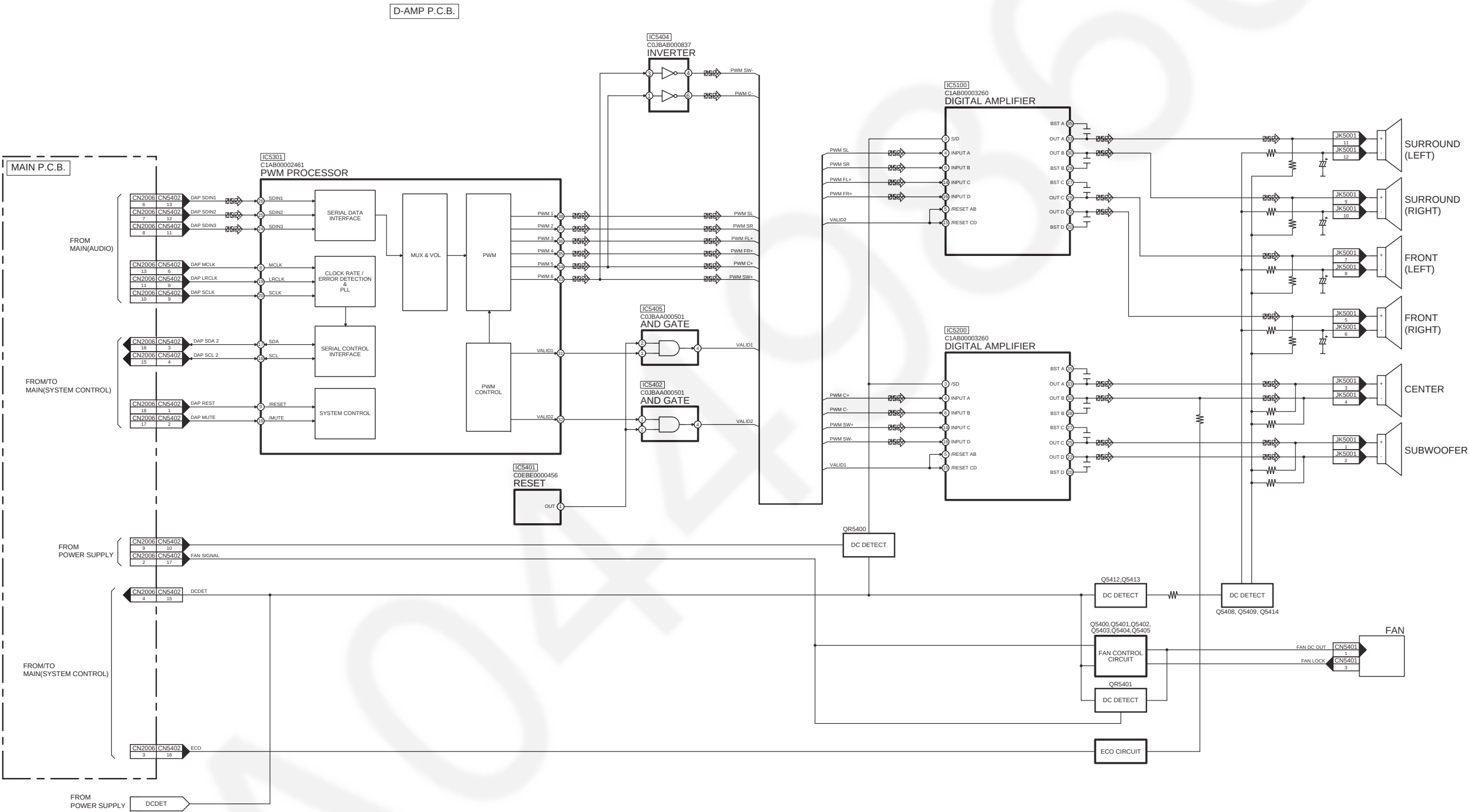
SA-PT480EB/EG DIGITAL AUDIO BLOCK DIAGRAM
