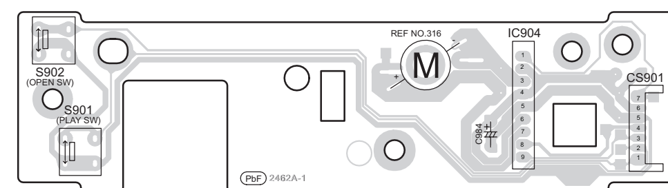
J TRAY LOADING P.C.B. (REP4238A)
