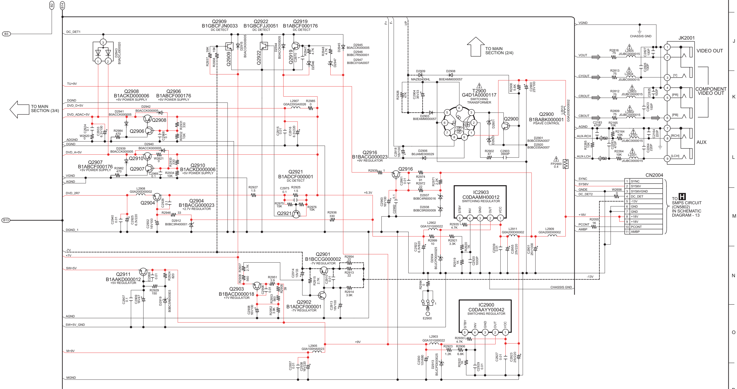
SA-PT250GCP MAIN CIRCUIT
