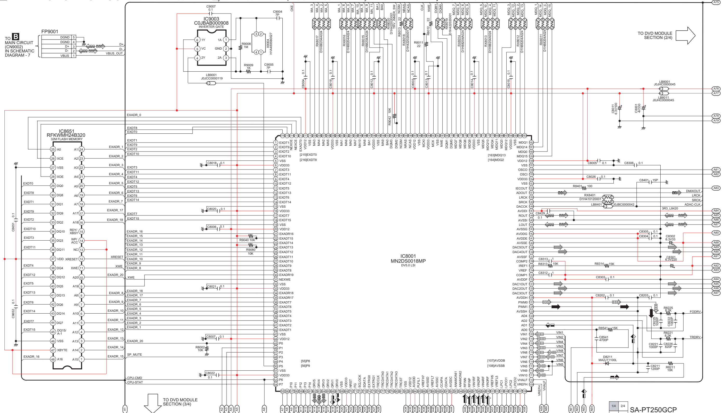
SCHEMATIC DIAGRAM - 1
