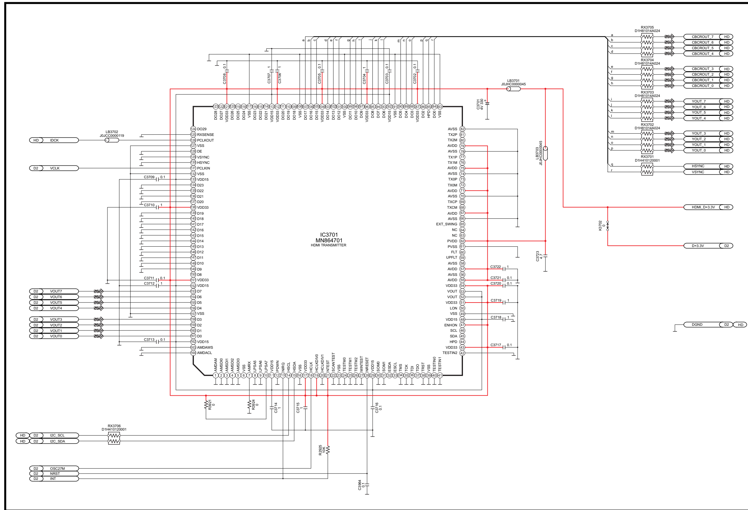
SA-HT995GC/GS/GCS HDMI MODULE CIRCUIT (UP)
