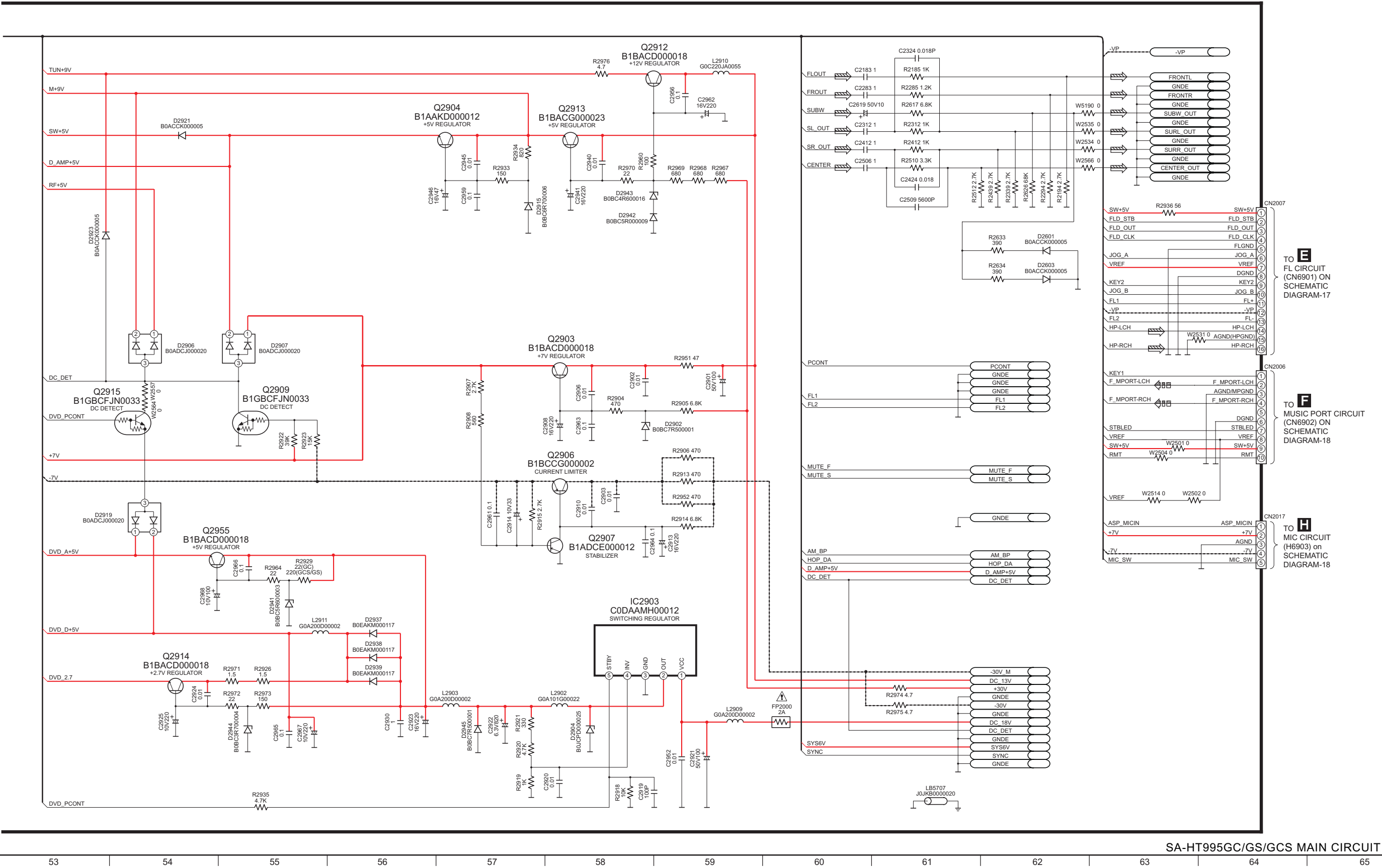
SCHEMATIC DIAGRAM-12
