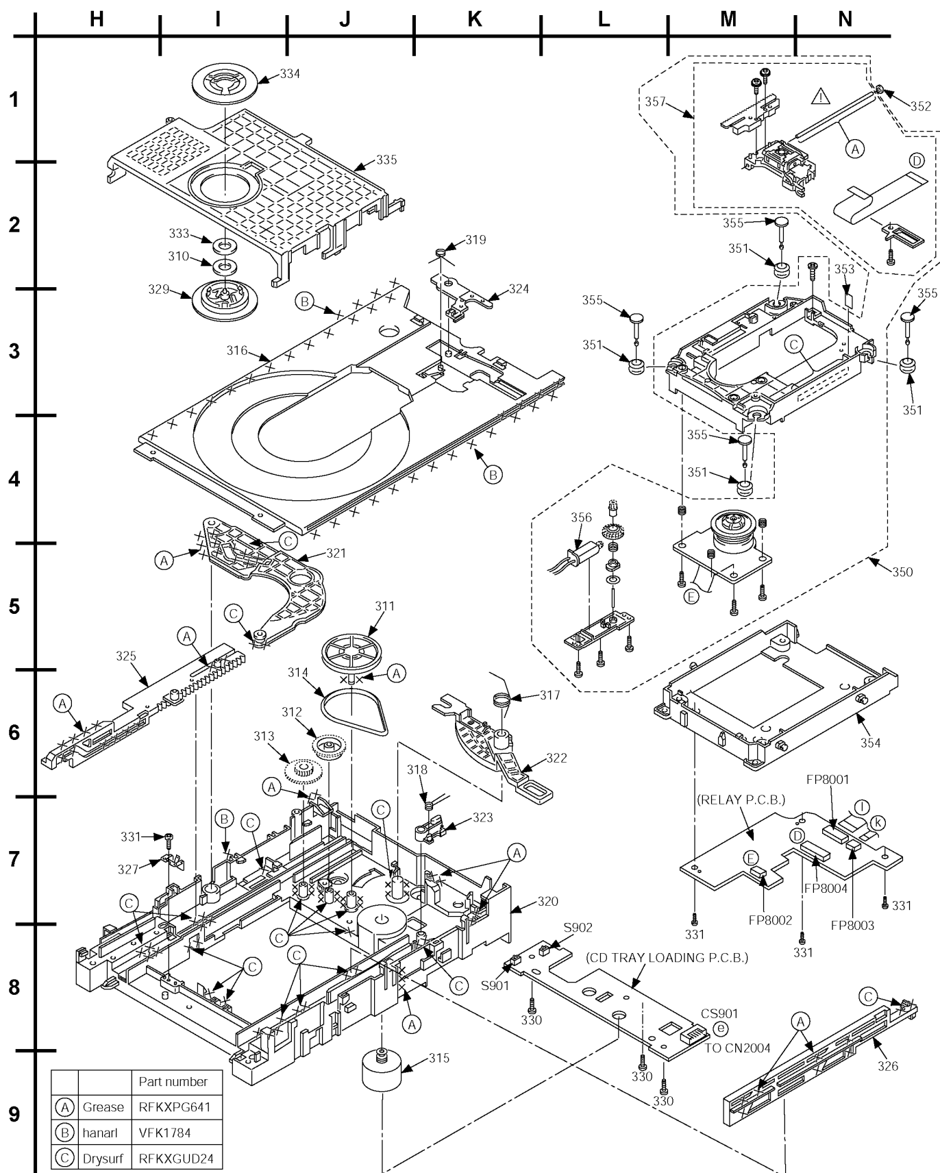
SA-HT995GC/GCS/GS DVD MECHANISM UNIT DRAWINGS
