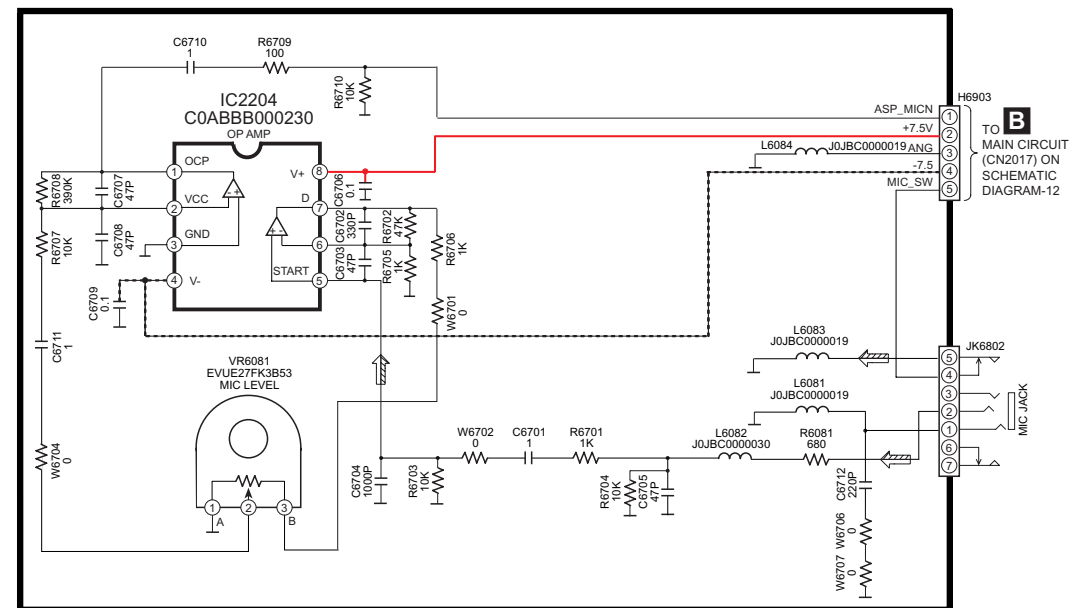
H MIC CIRCUIT
