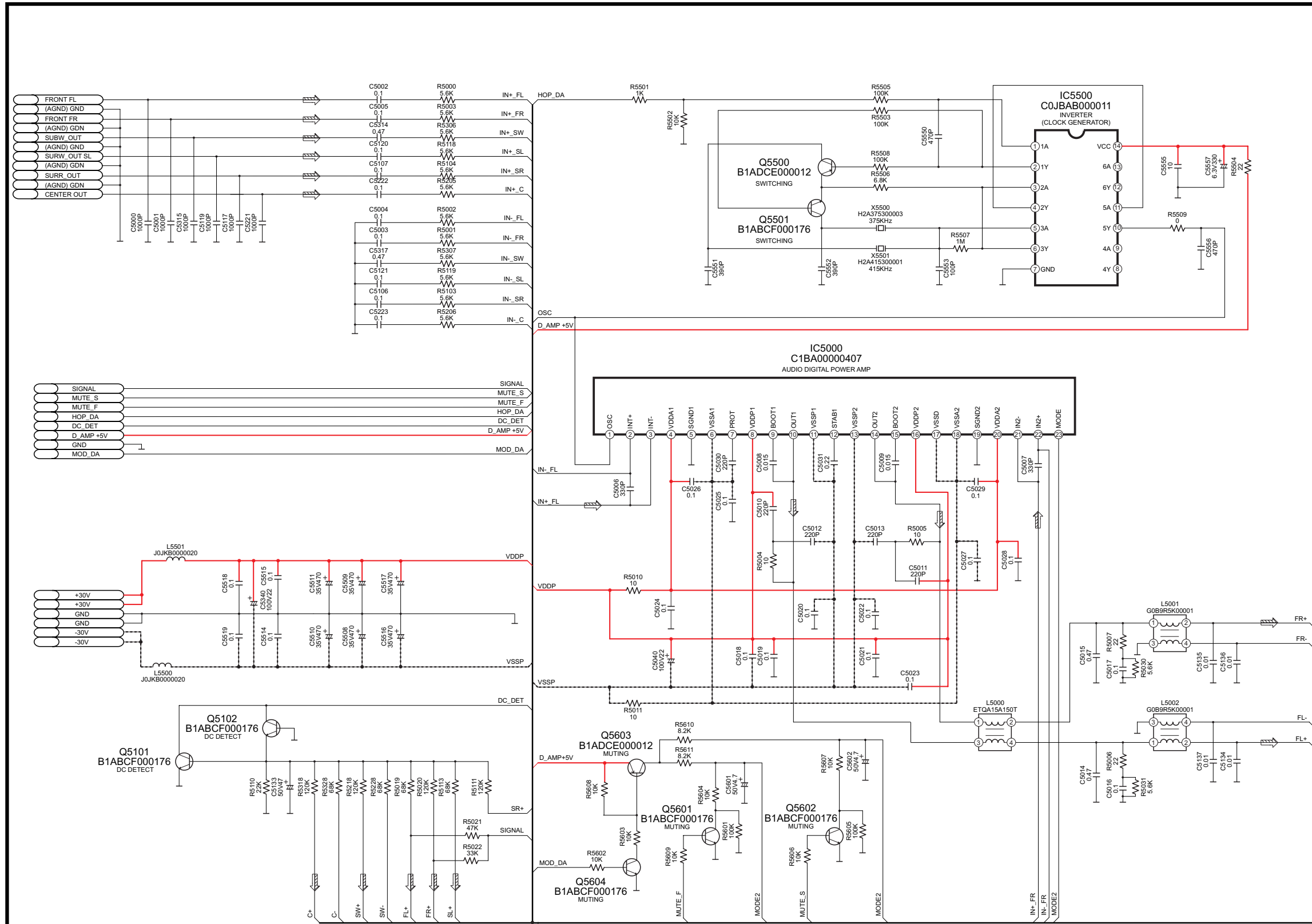
SA-HT995GC/GS/GCS POWER(DIGITAL AMP) CIRCUIT
