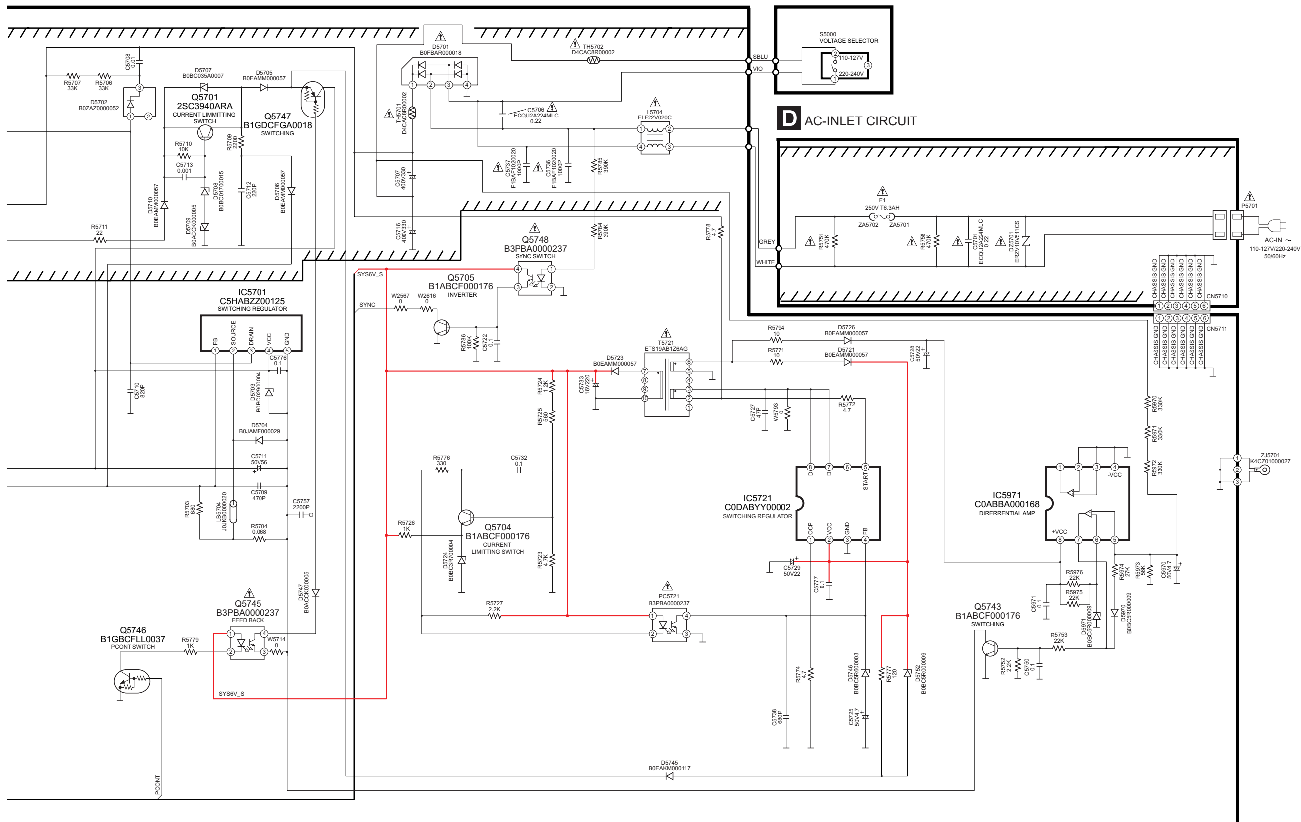
SCHEMATIC DIAGRAM-16
