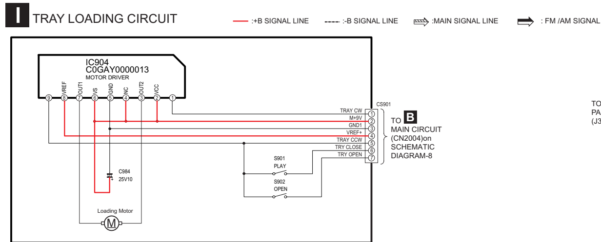
SCHEMATIC DIAGRAM-18
