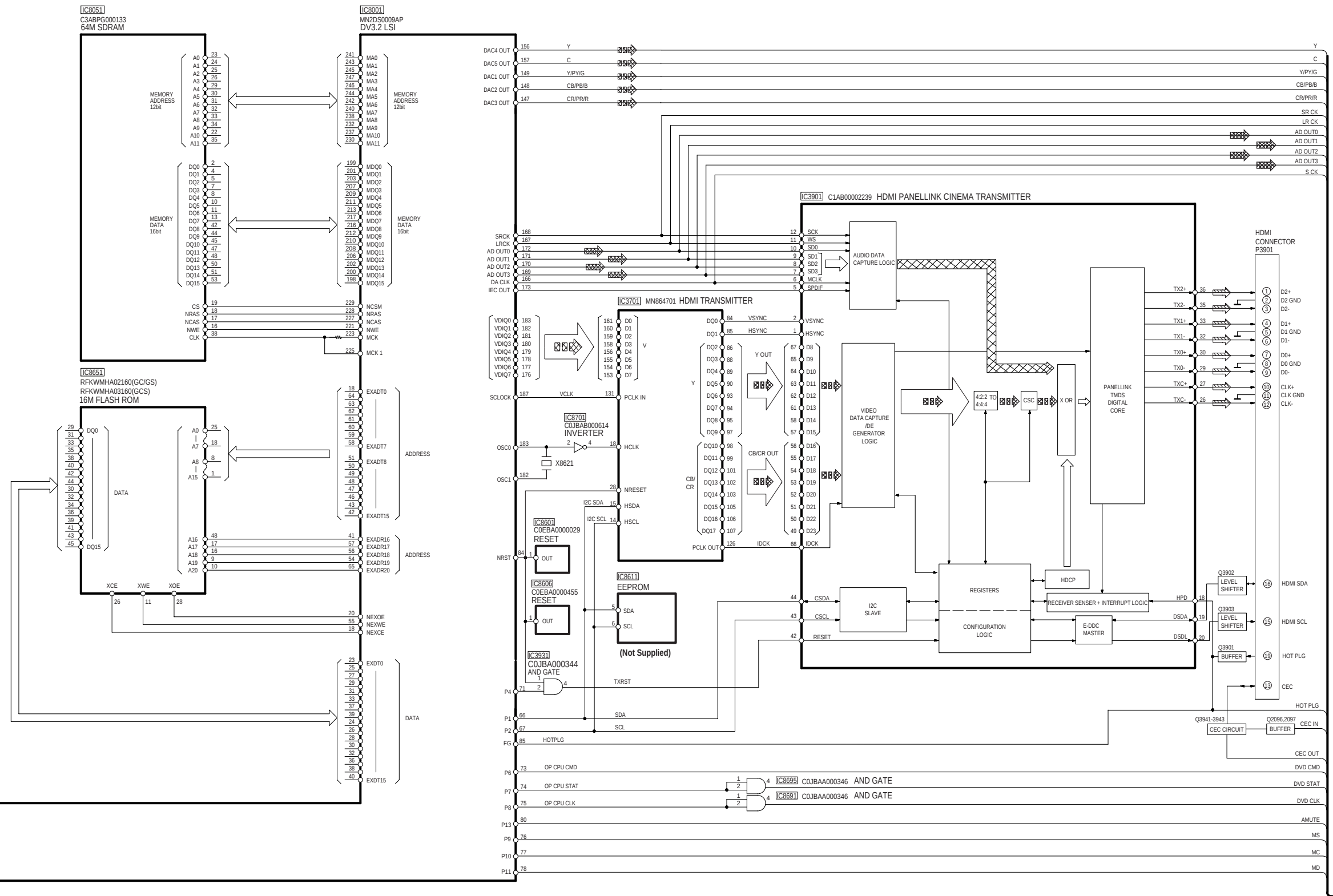
SA-HT895GC/GCS/GCT BLOCK DIAGRAM
