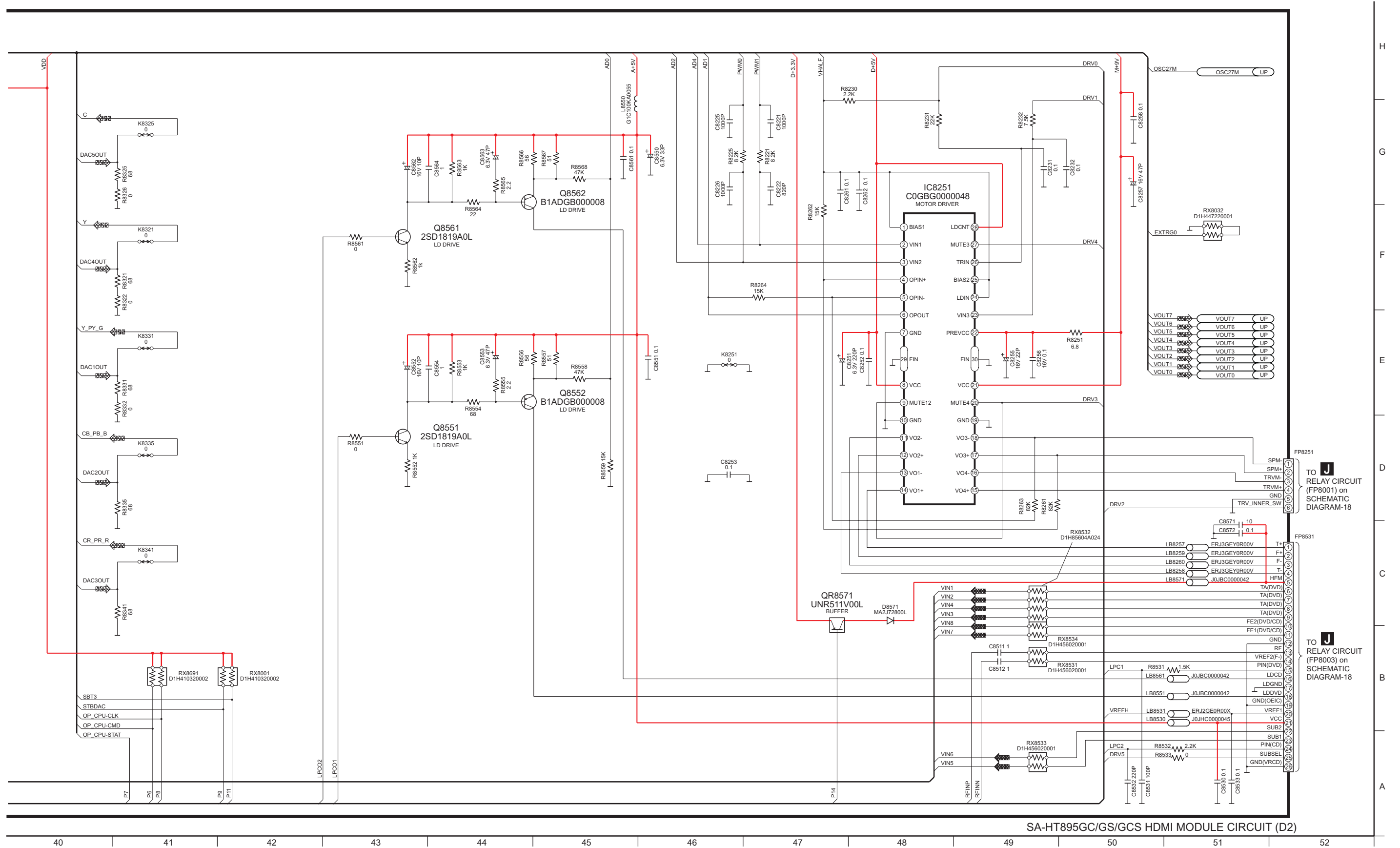
SCHEMATIC DIAGRAM-5
