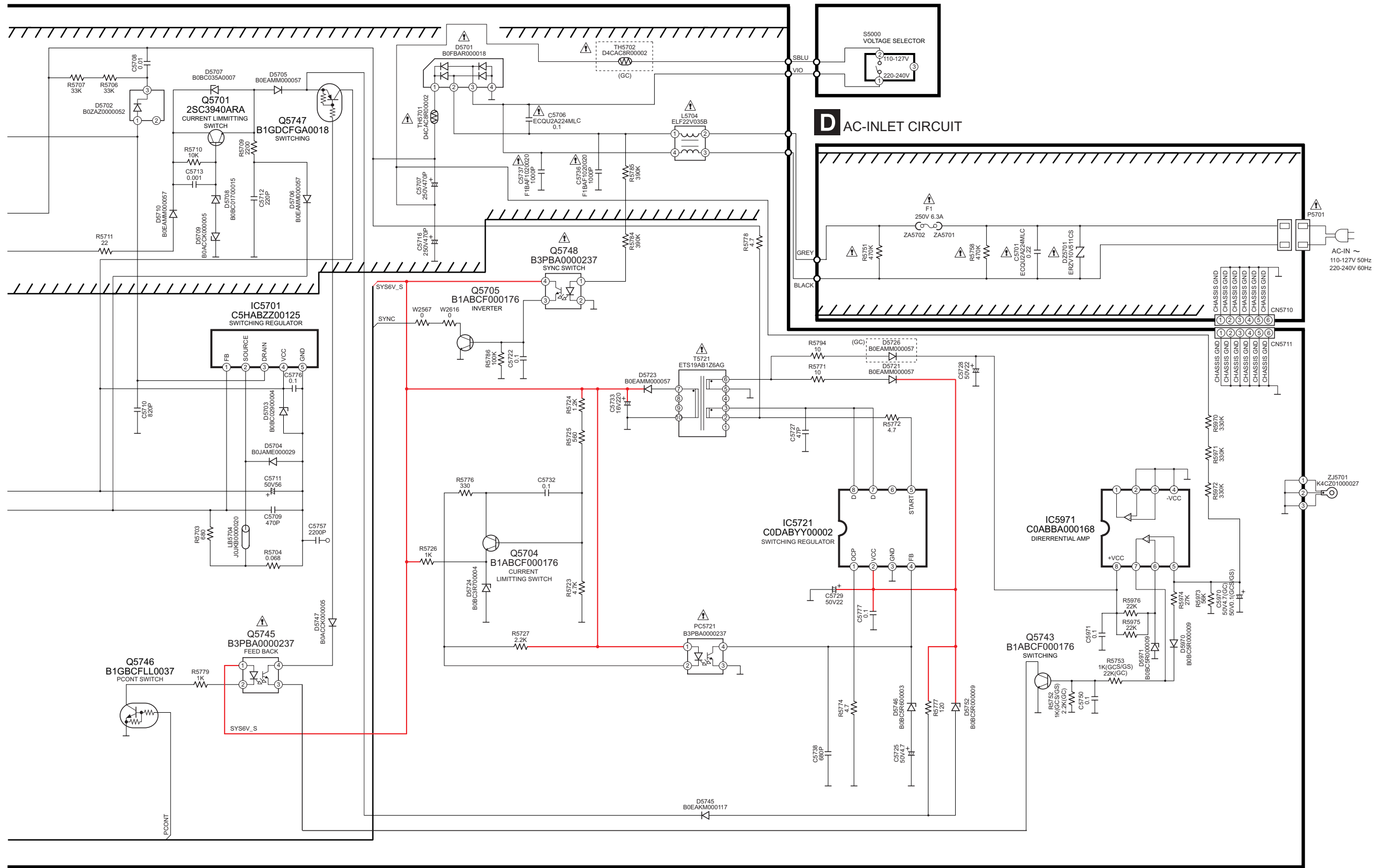
SA-HT895GC/GS/GCS POWER(SMPS)/AC-INLET CIRCUIT/VOLTAGE SELECTOR
