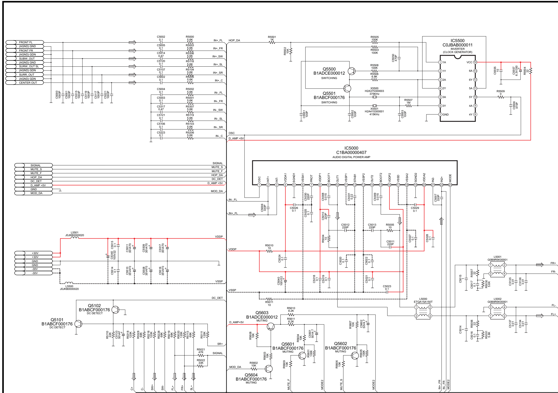
SA-HT895GC/GS/GCS POWER(DIGITAL AMP) CIRCUIT
