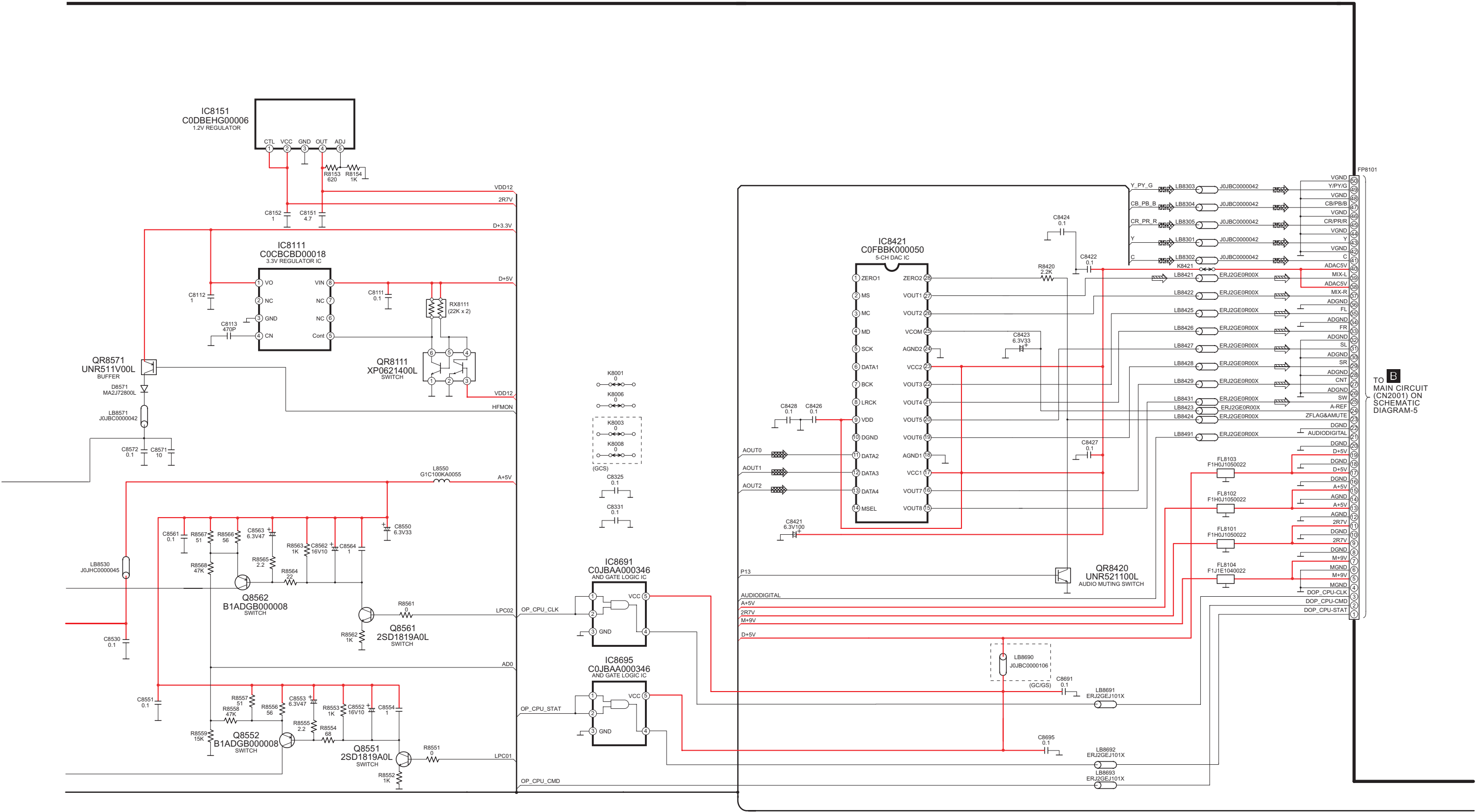
SA-HT340GC/GCS/GS DVD MODULE (DV3.2) CIRCUIT
