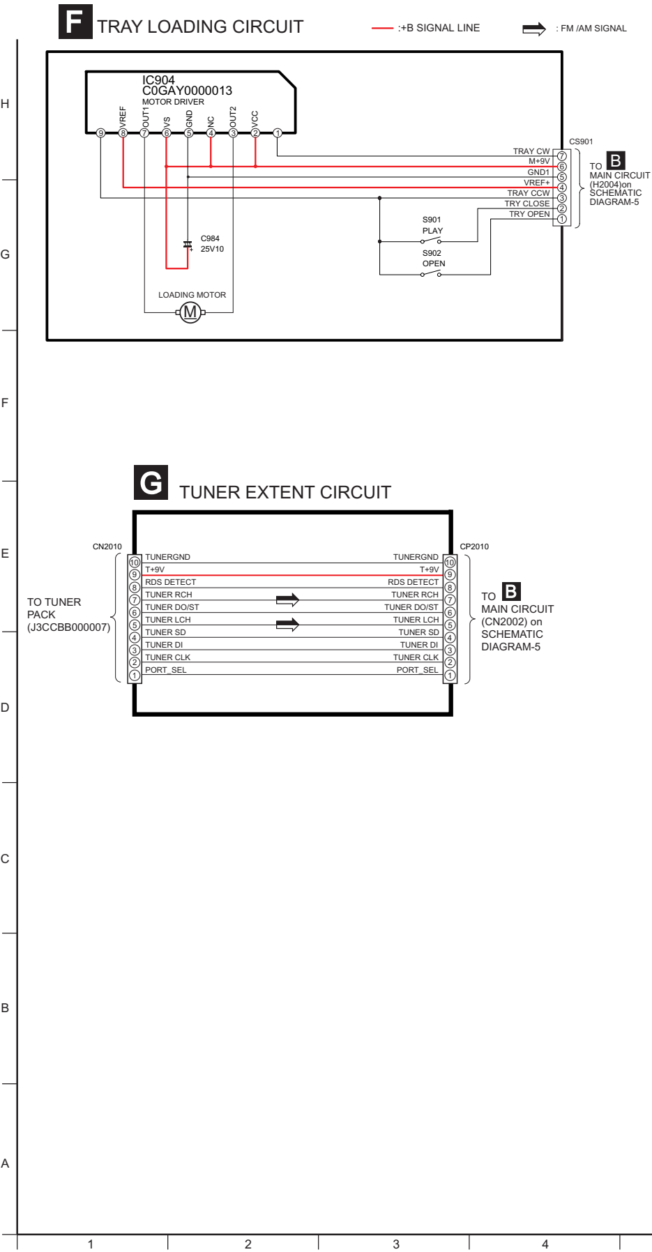
SCHEMATIC DIAGRAM-11
