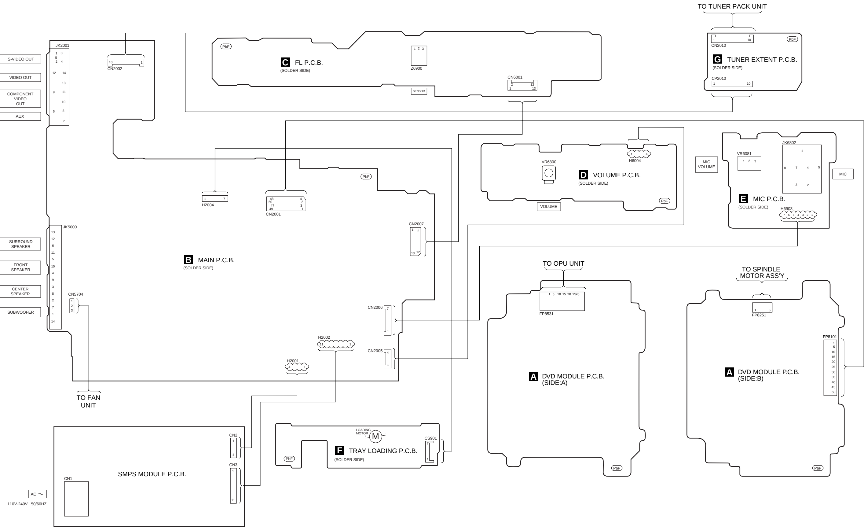
SA-HT340GC/GCS/GS WIRING CONNECTION
