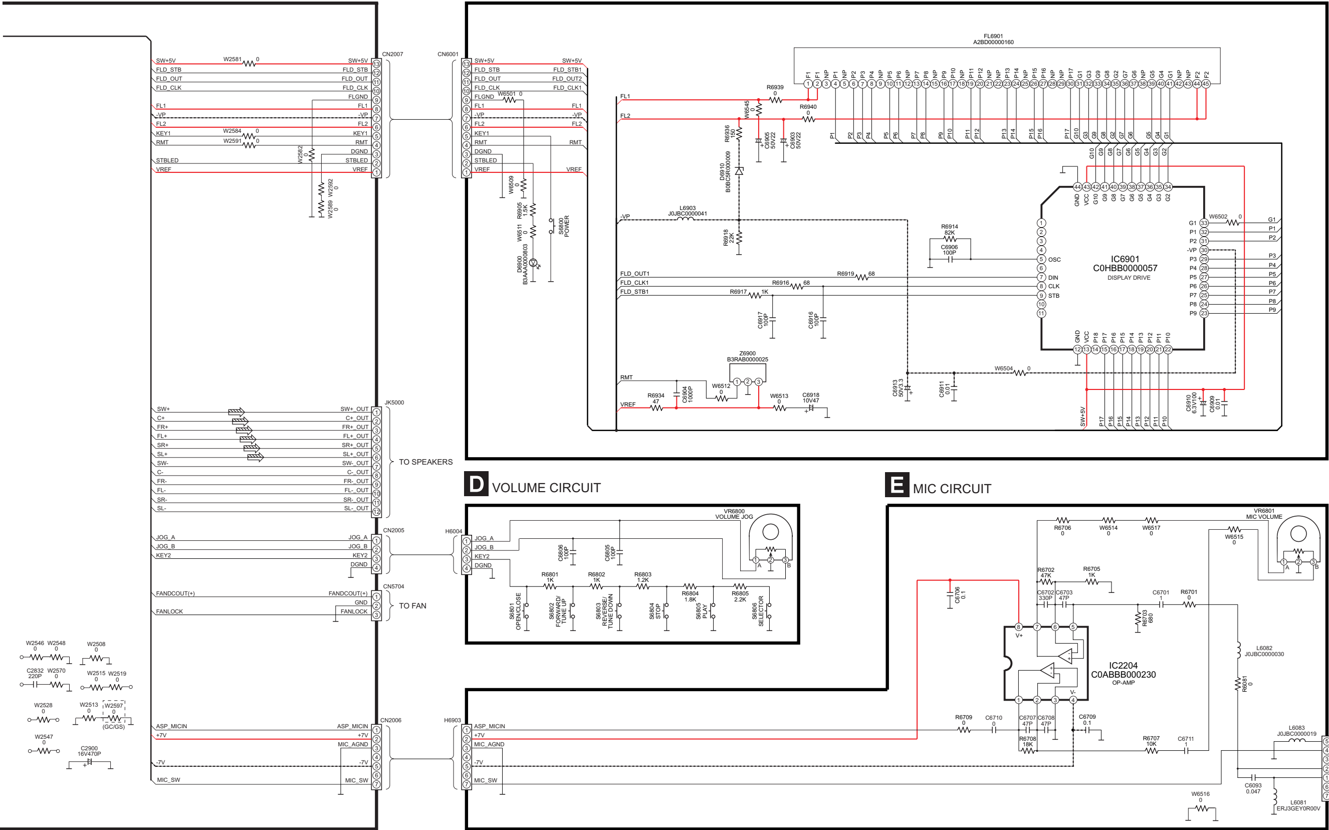
SA-HT340GC/GCS/GS MAIN/FL/VOLUME/MIC CIRCUIT
