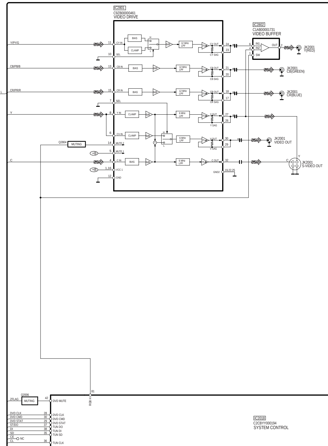
SA-HT340GC/GCS/GS BLOCK DIAGRAM
