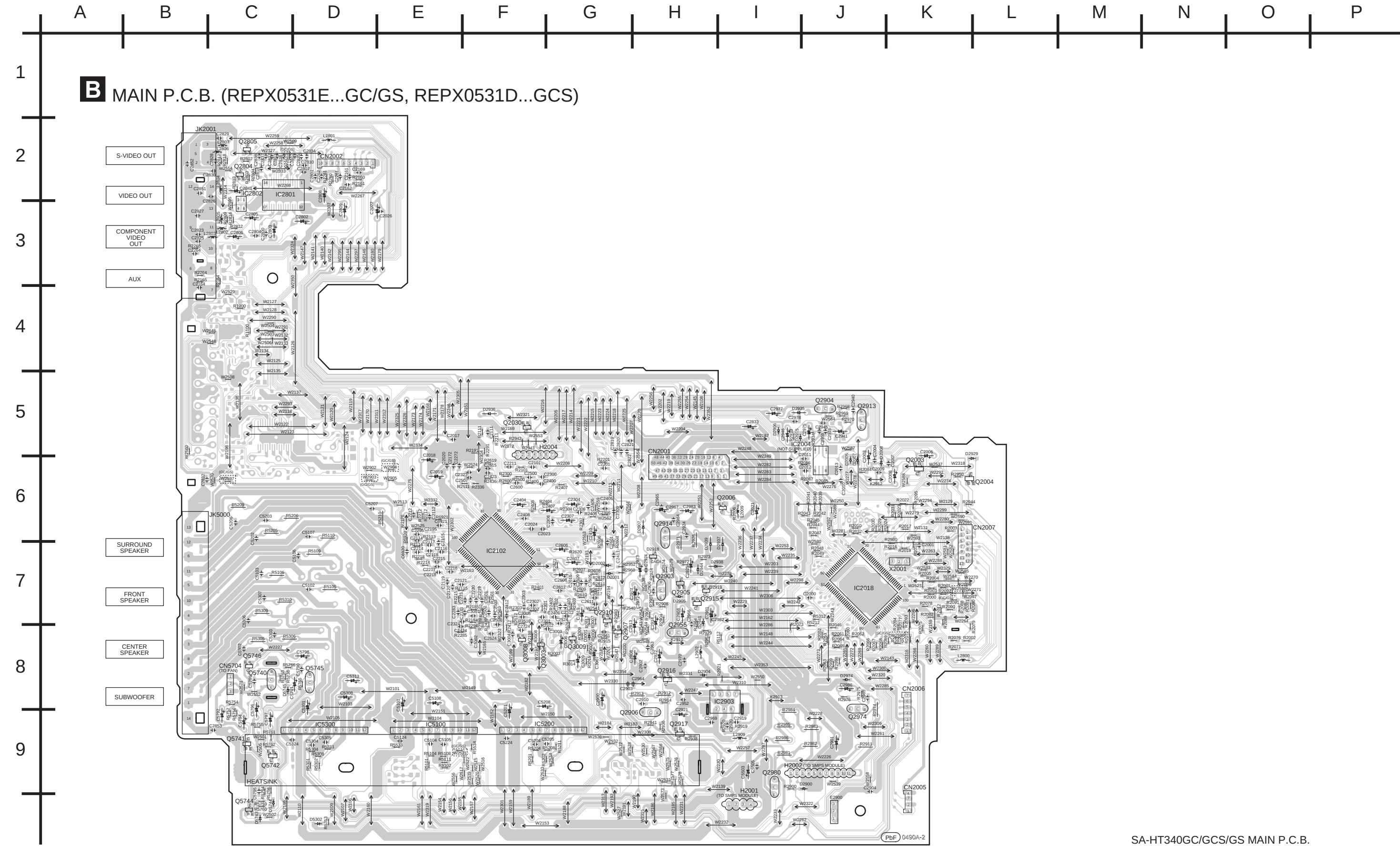
SA-HT340GC/GCS/GS MAIN P.C.B.
