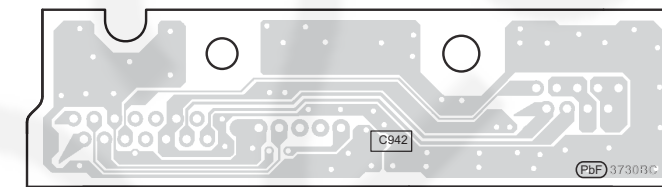
C BRIDGE P.C.B. (REP5053QC...HC395EG) (REP5053SC...HC397EB/EG)
