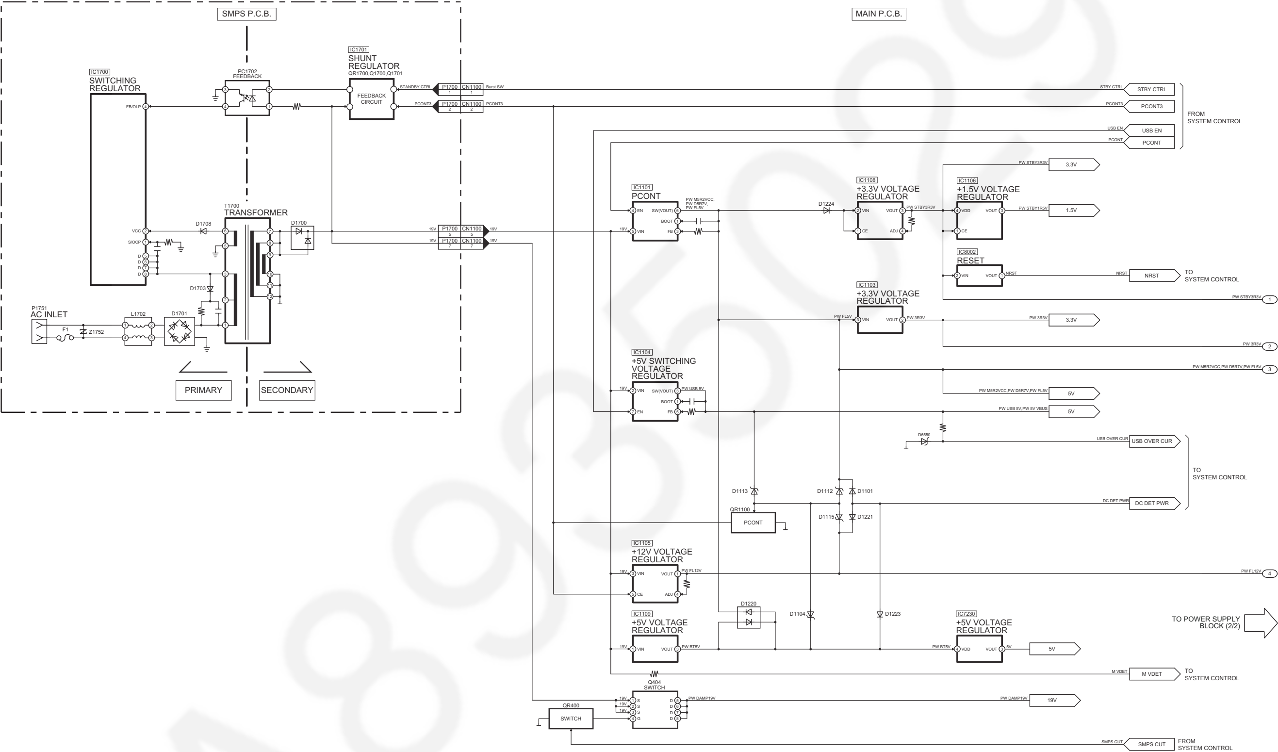
SC-HC395EG,SC-HC397EB/EG POWER SUPPLY (1/2) BLOCK DIAGRAM
