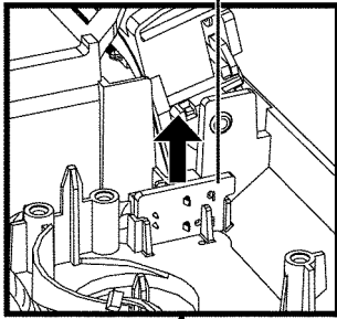
(Step 5) iPod Open Switch P.C.B.
