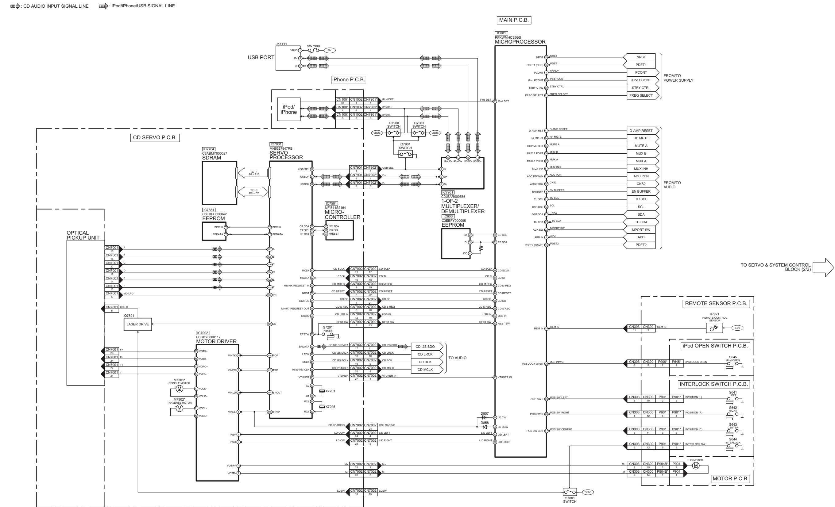
SC-HC35GS/GSX/GT SERVO & SYSTEM CONTROL (1/2) BLOCK DIAGRAM
