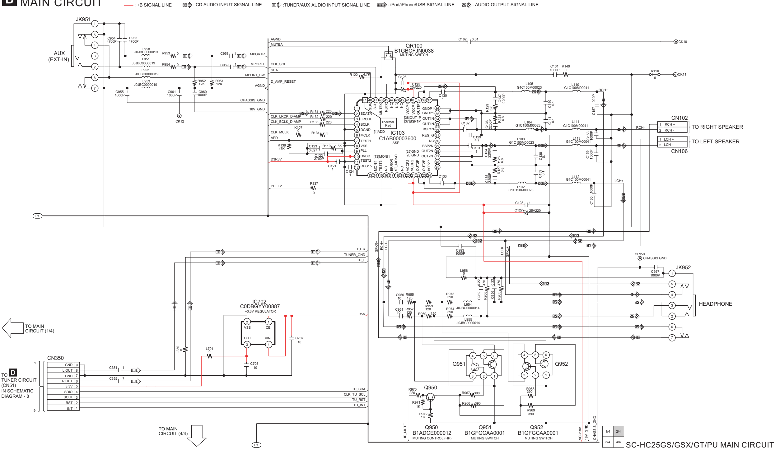
SCHEMATIC DIAGRAM - 4
