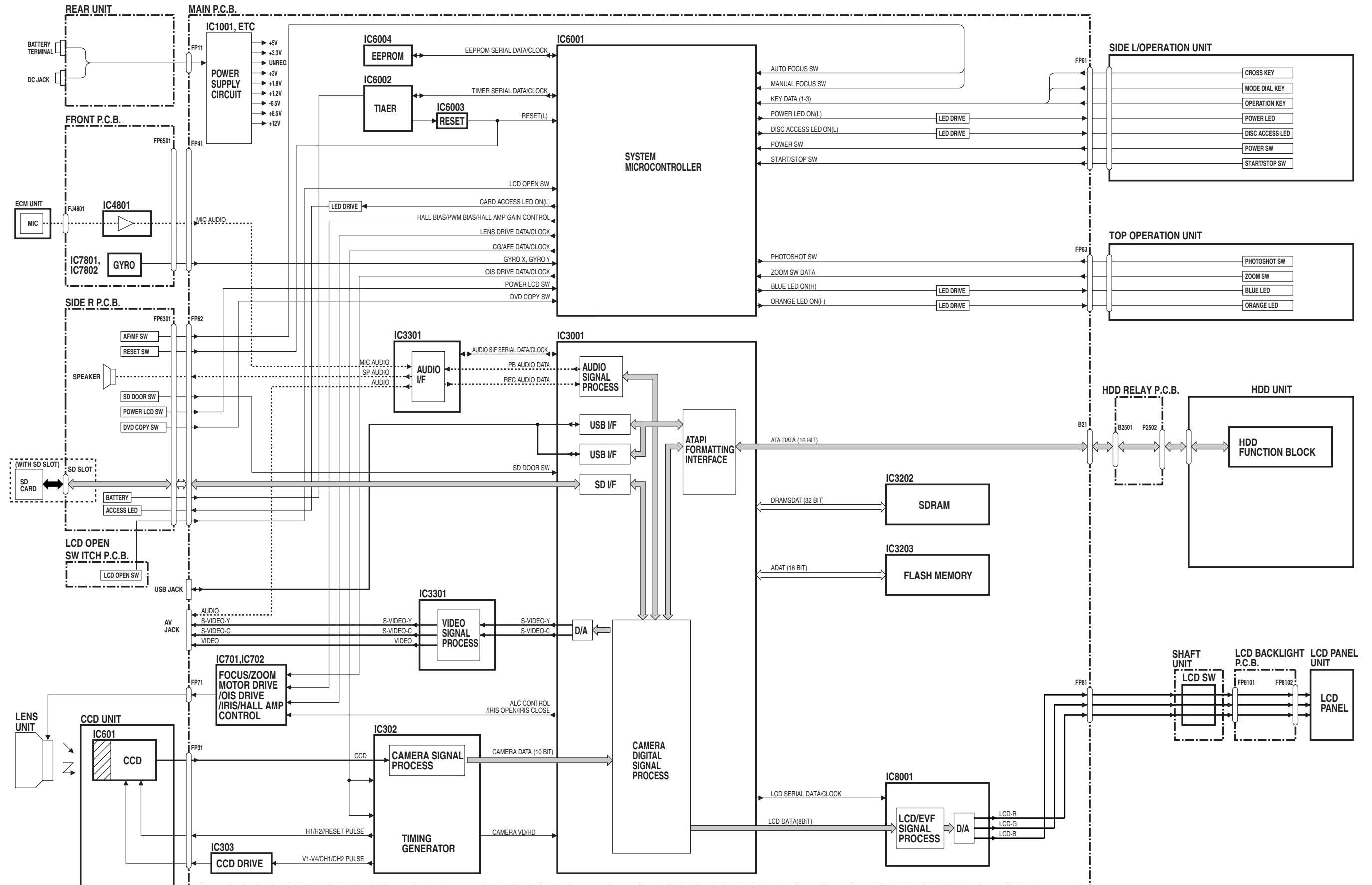
OVERALL BLOCK DIAGRAM SDR-H20E/EB/EE/EF/EG/EP/GC/GN, SDR-H21EE/GC, SDR-H28GK, SDR-H29GK
