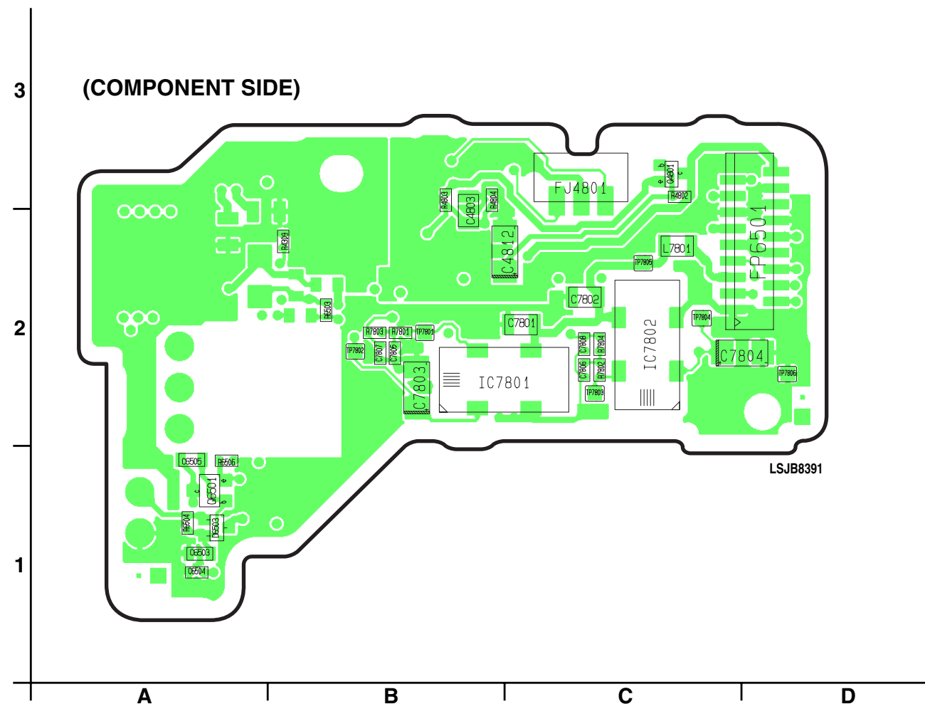
Parts Location
