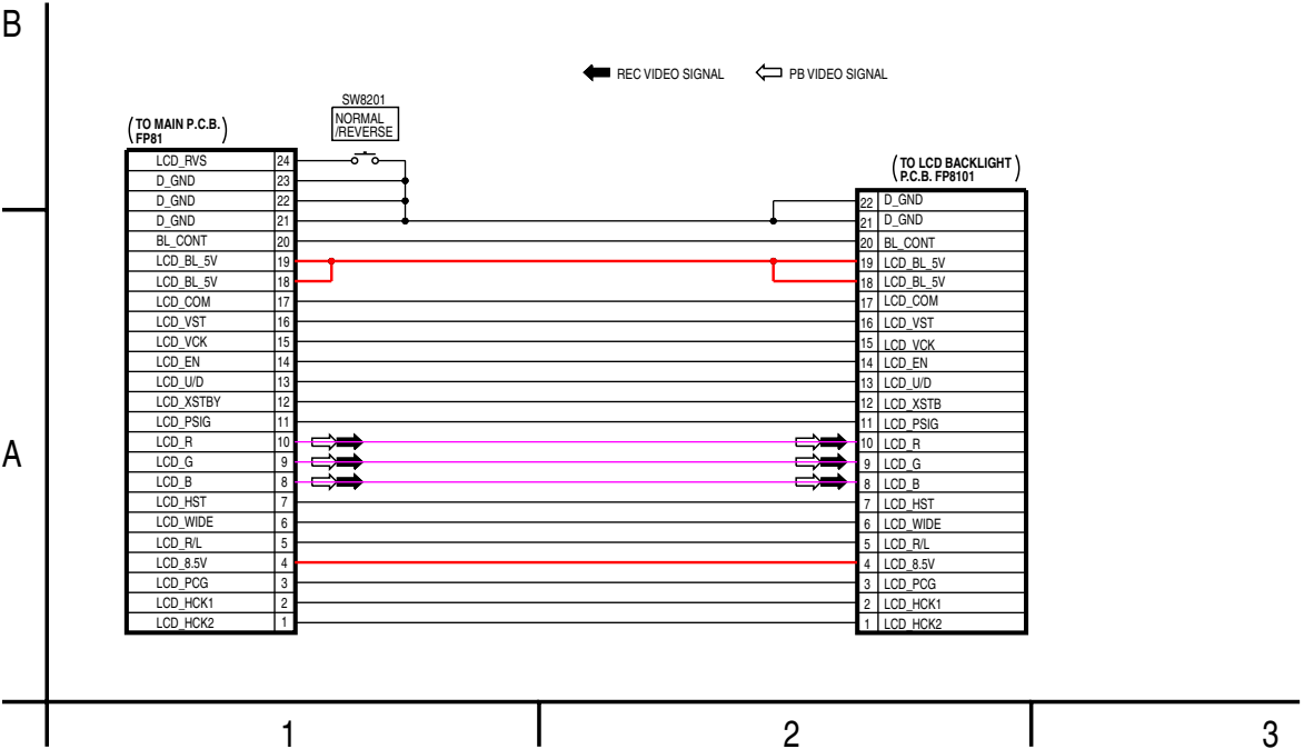
HDD RELAY FPC SCHEMATIC DIAGRAM “FOR REFERENCE ONLY”
