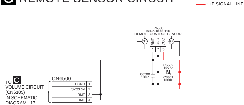
SCHEMATIC DIAGRAM - 20
