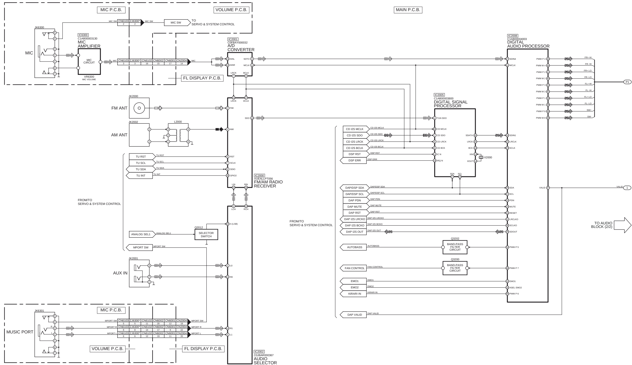
SA-MAX700GS AUDIO (1/2) BLOCK DIAGRAM
