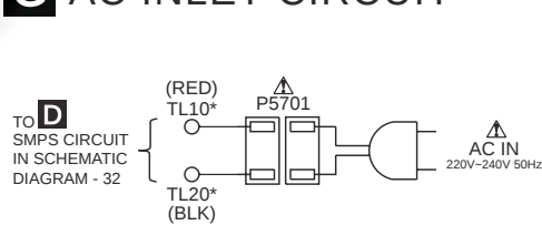
G AC INLET CIRCUIT
