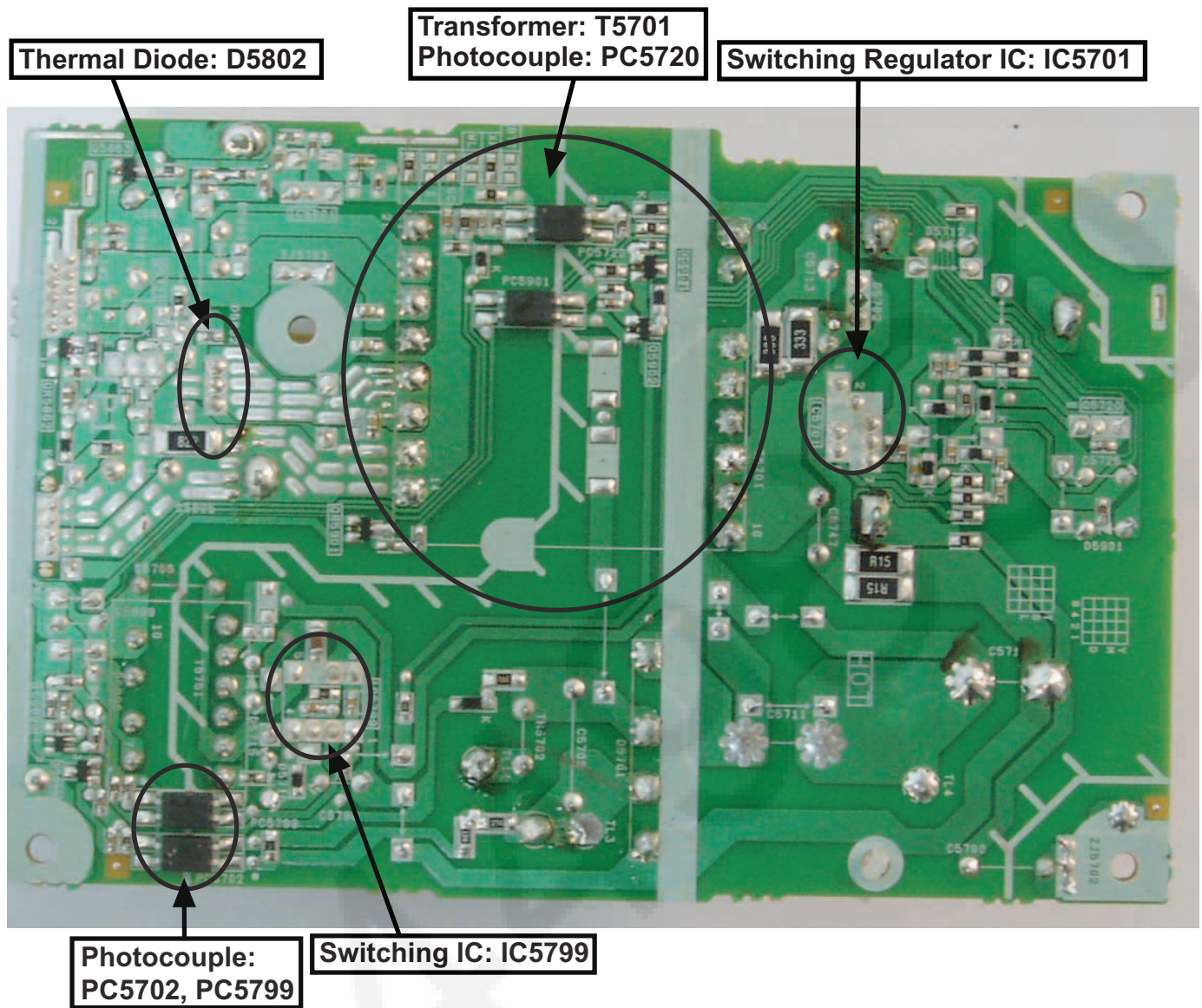
Figure 1. SMPS P.C.B.
