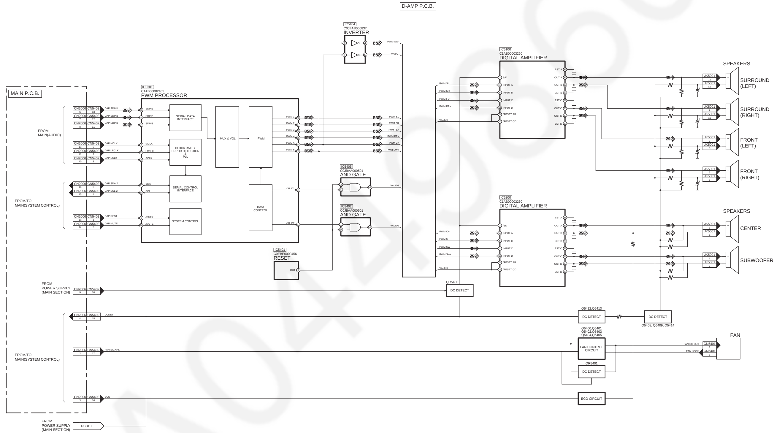
SA-BT735EB/EE/EG/EP DIGITAL AUDIO BLOCK DIAGRAM
