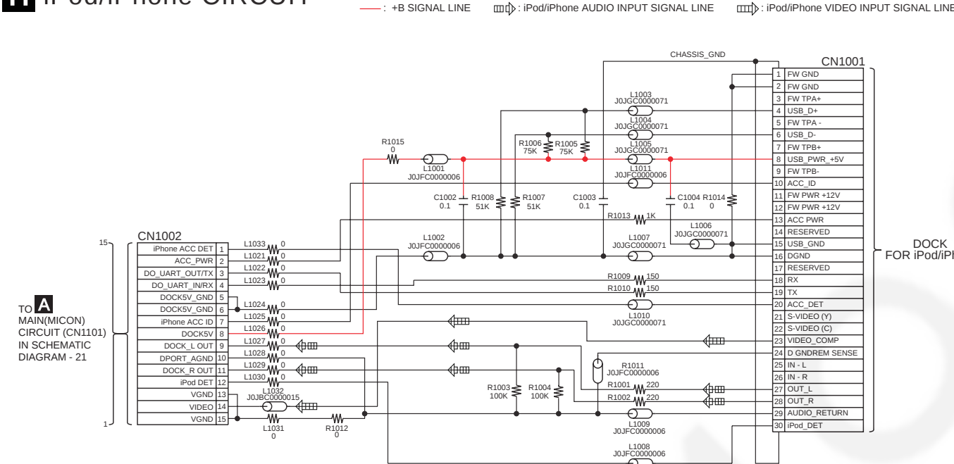
SCHEMATIC DIAGRAM - 34
