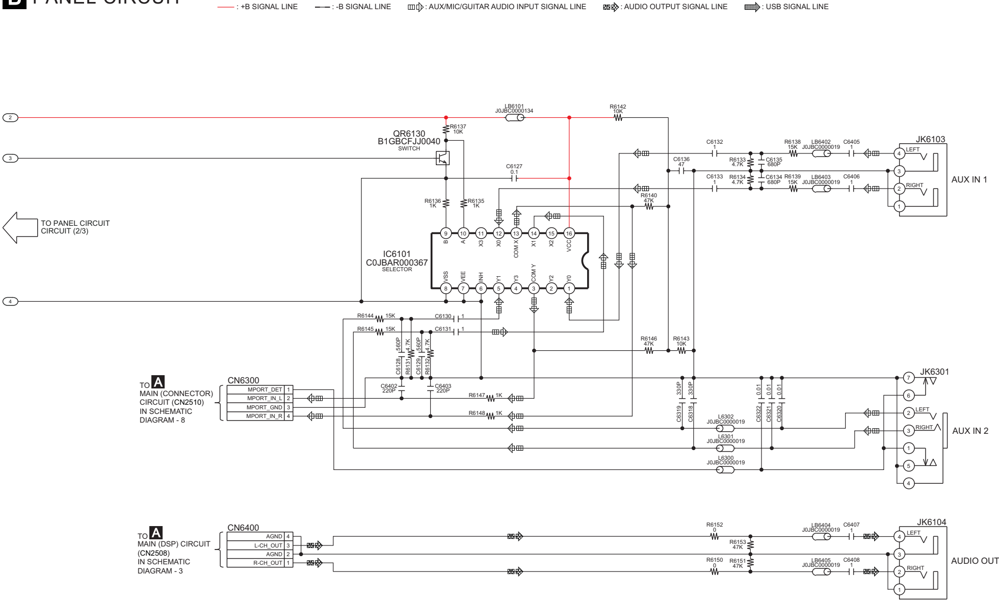
SCHEMATIC DIAGRAM - 11
